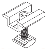
Mid Clamp
